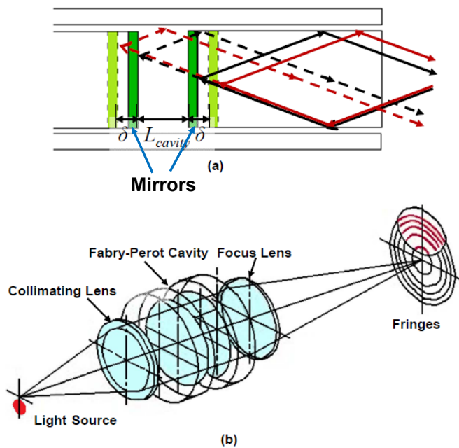
Fig. 8. The Fabry-Perot sensing principle and its light propagation in Fabry-Perot cavity (a) and one type of implementation (b) [46] ©IEEE 2011.
